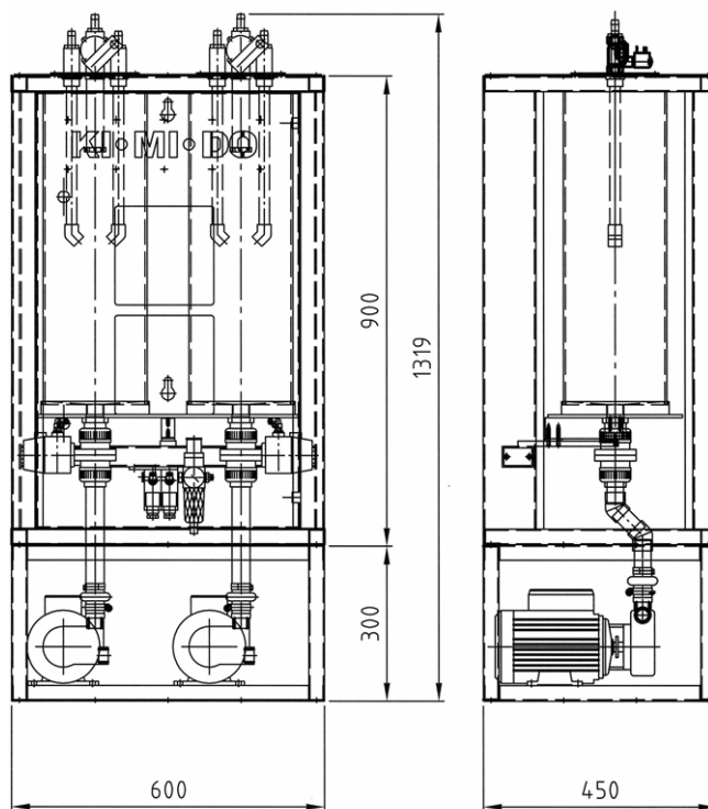
Dimensions in [mm] according drawing no. 0300.1200.60.01
