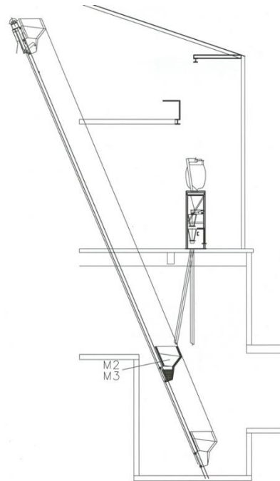
Side view PFW 10 with bucket conveyor and down pipes with discharge into the skip hoists
