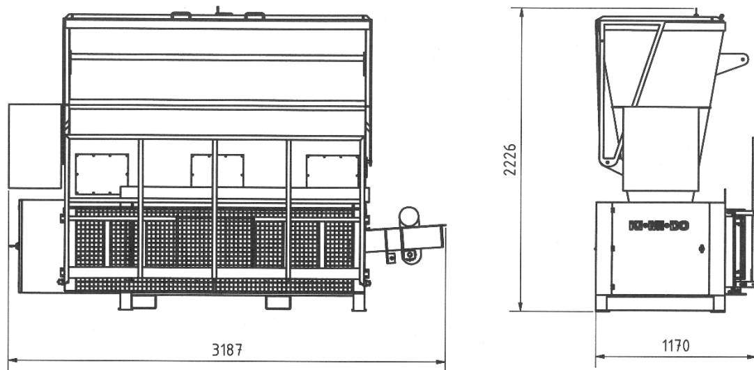
Dimensions FS 1700/400 during transport according 0700.500.60.01.2
