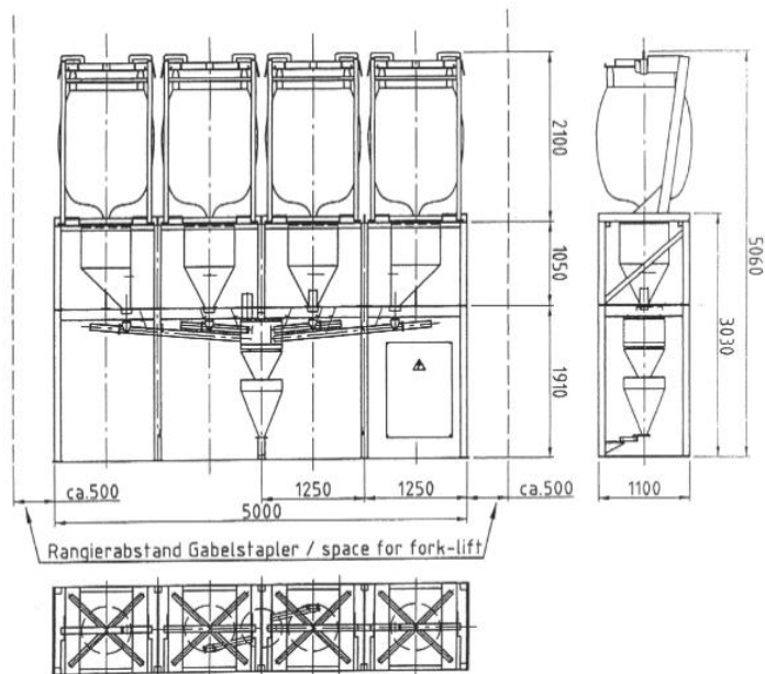
Dimensions FD . WS (weighing vessel)
