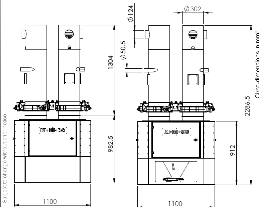
Fig. Dimensions PDE 75/4 – for 1 – 4 components
