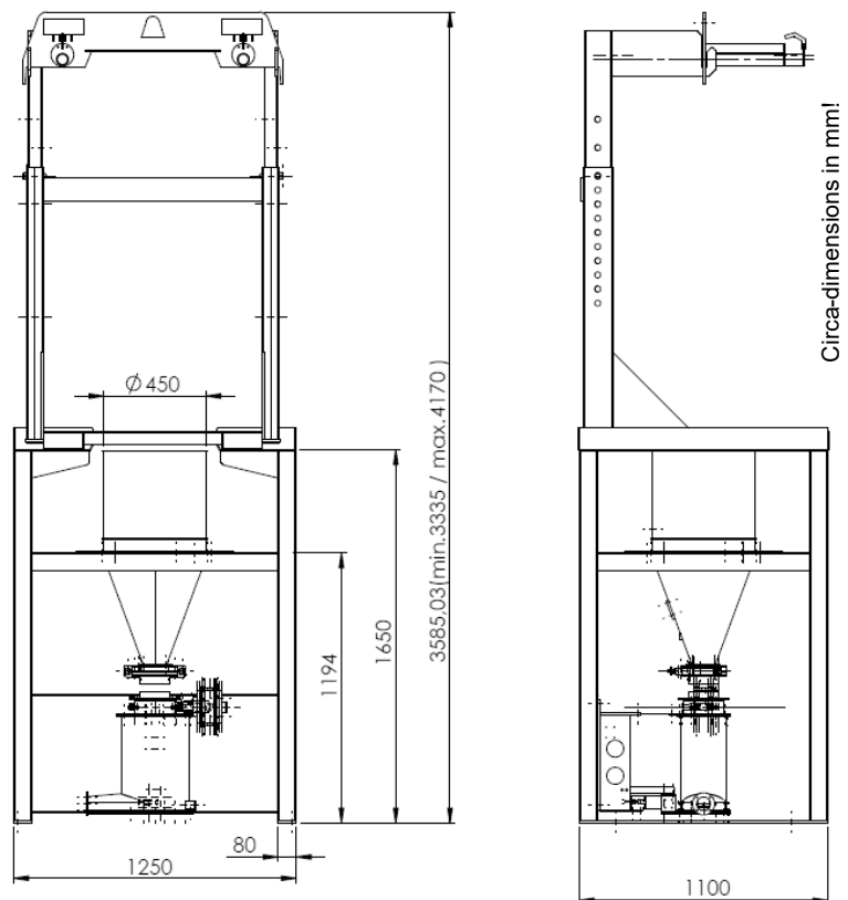
Fig. Dimensions Big-Bag conveying unit for 1 component
