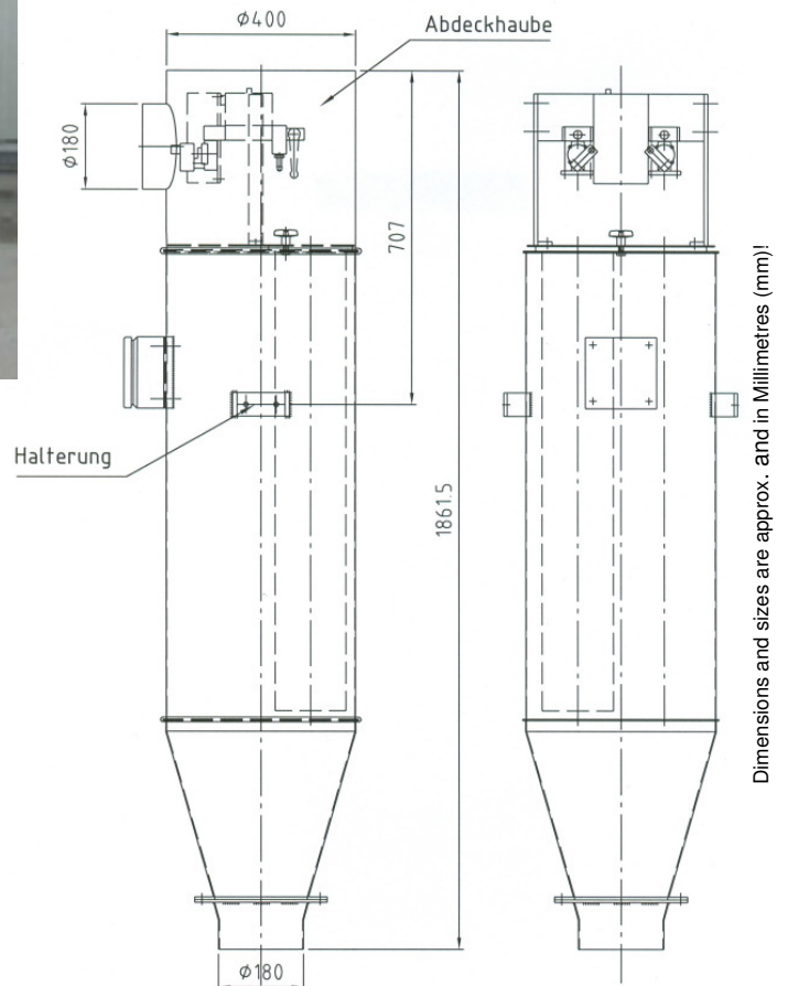
Fig.: Dimensions dust collector size VII 7.5 m 2
