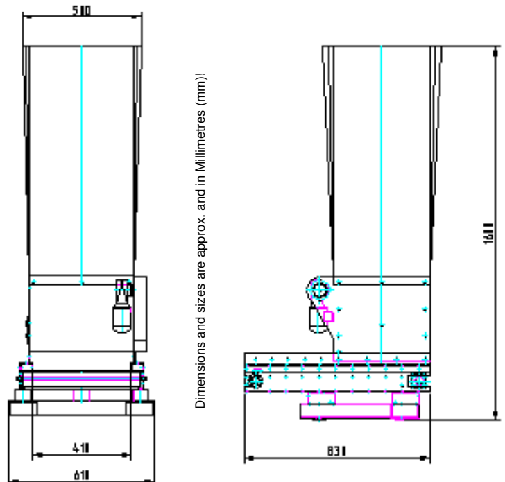
Fig.: Dosing machine for fibres F-4R/400
