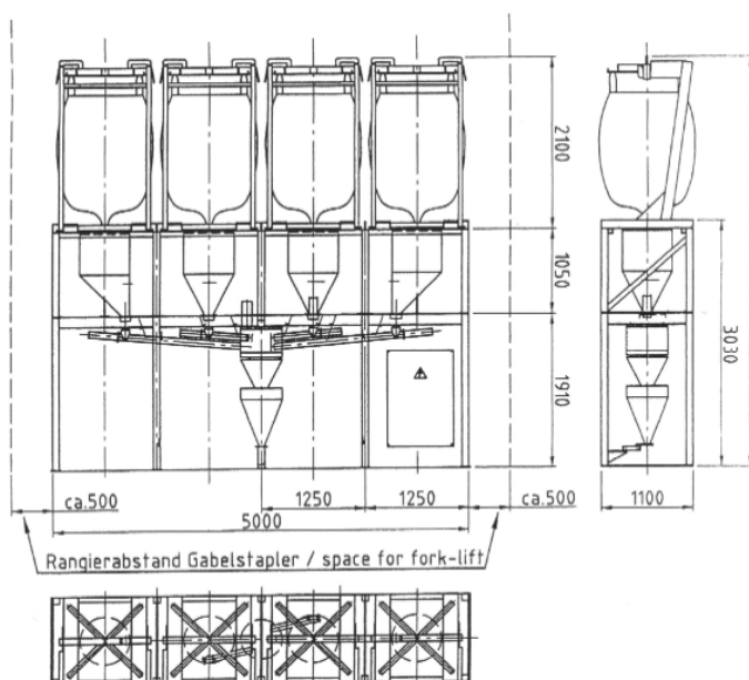
Fig. Dimensions FD . WS (weighing vessel)
